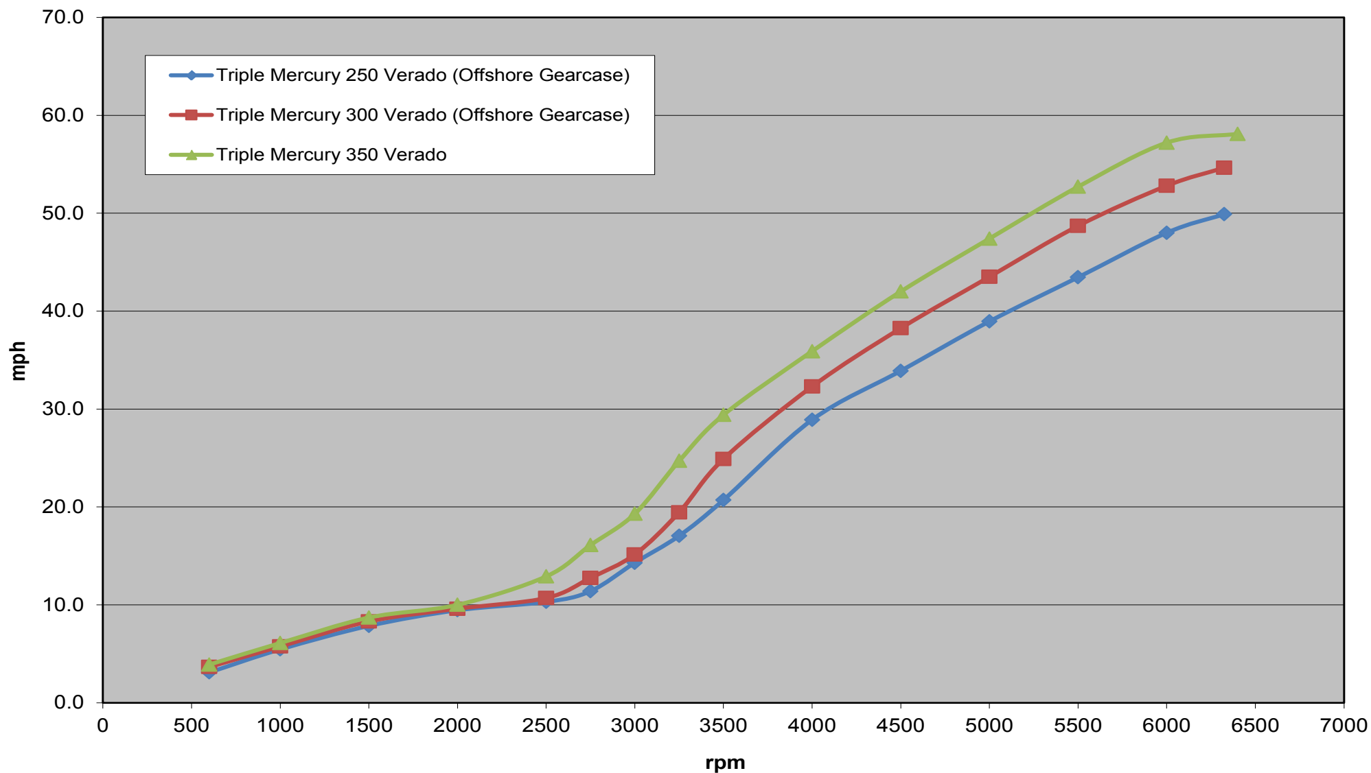
370 Outrage Engine Comparison Graph
