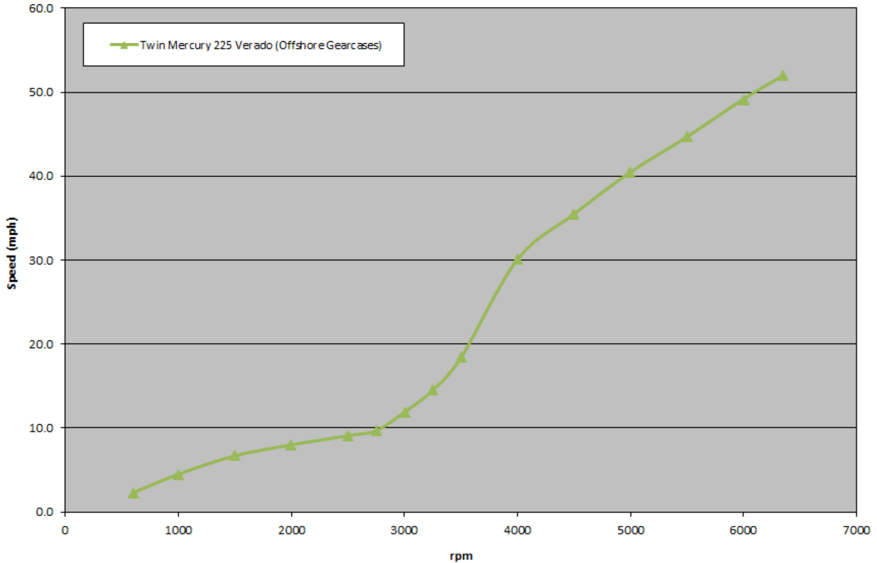
250 Outrage 2016 Engine Comparison Graph
