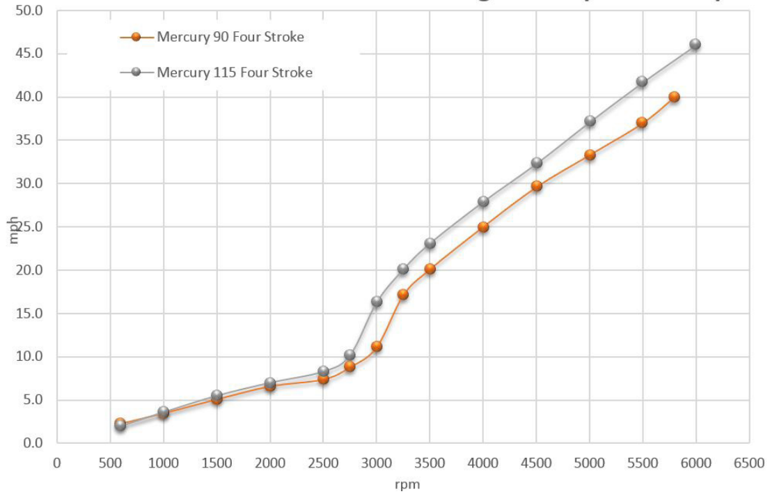
170 Montauk 2018 Engine Comparison Graph
