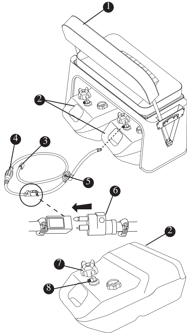
Fuel tanks Fig. 3.2.1
