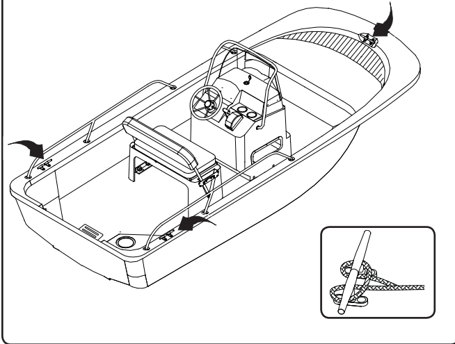
Cleat Locations Fig. 2.16.1
