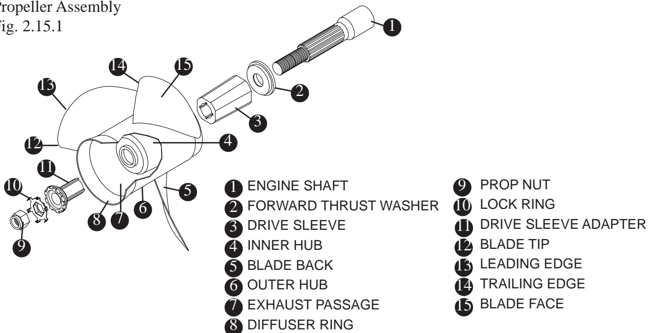
Propeller Assembly
