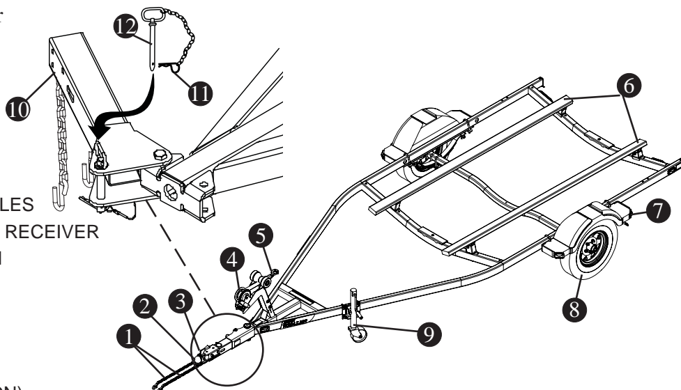
Single Axle Bunk Trailer Fig. 2.18.1
